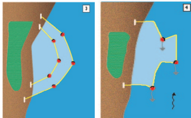
Figure 4 displays a site with a one directional current of 3 feet per second or less, running parallel to the shore line. Sites that have moving water, currents, waves, or tides, require the installation of a Type 2 DOT barrier. This type of barrier is specifically designed for areas near dredging projects, rip rap installation, and DOT roadwork and construction. In areas with flowing water, accurate anchor installation will ensure that the curtain bears against changes in wind or current.
