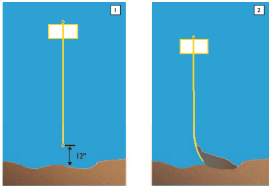
Figure 1 illustrates the standard practice of installing a barrier so that the lower edge of the skirt is about 12 inches from the bottom, with the ballast chain keeping the skirt more vertical in the water column. Depending on the site conditions, it is recommended that the curtain should be at least 25 feet from an outlet. This allows the sediment to settle naturally. If the lower edge of the curtain drapes at the bottom, silt will build up as shown in Figure 2. The buildup of silt may submerge the curtain, disturbing the settling process and sending sediment back into the water course upon removal.
