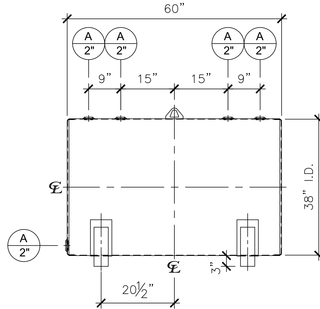
FRONT VIEW
