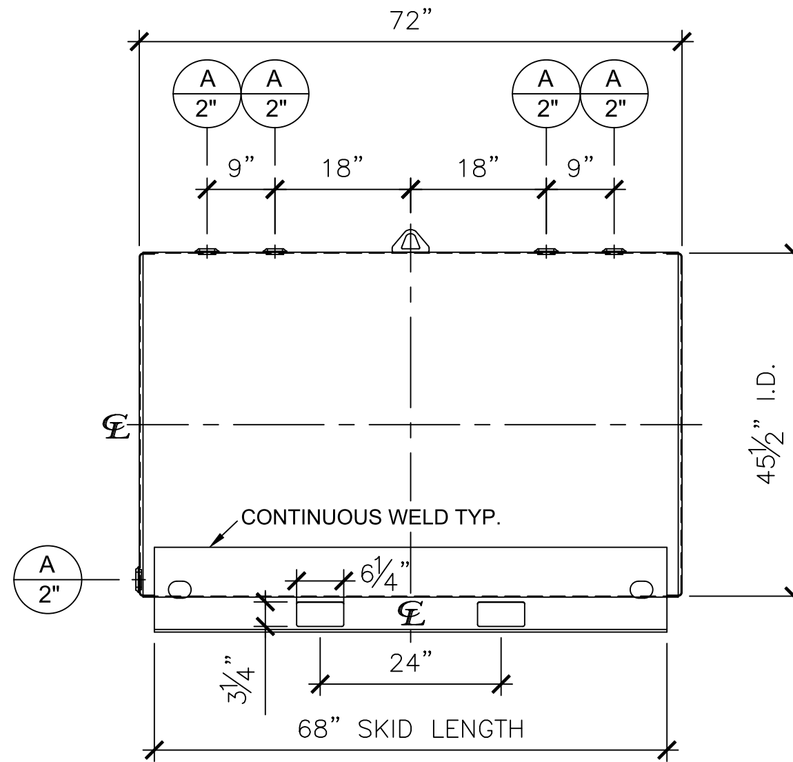
FRONT VIEW
