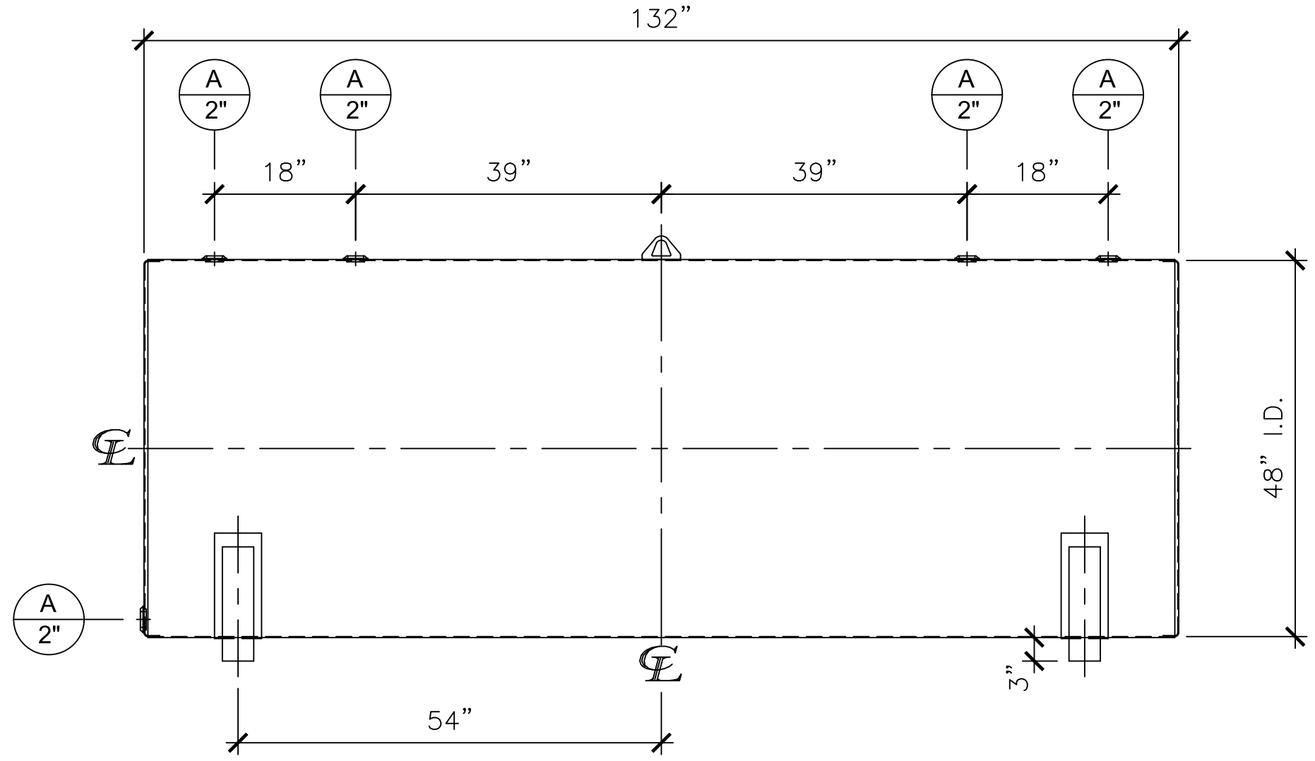
FRONT VIEW
