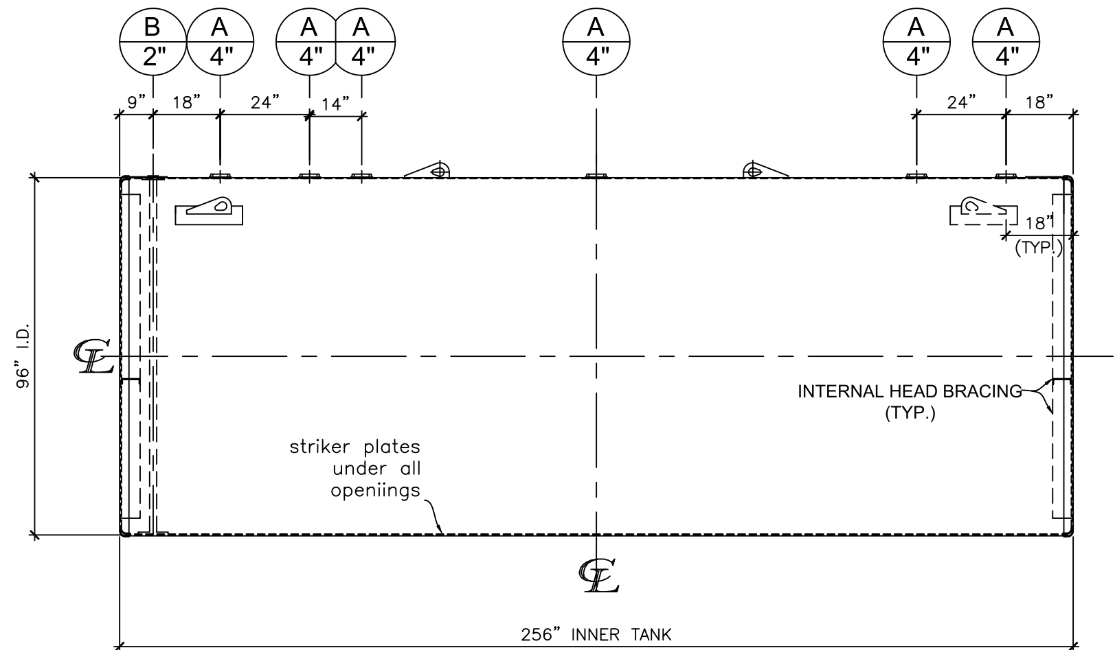
FRONT VIEW
