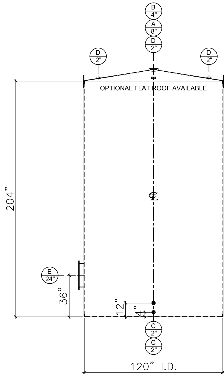
FRONT VIEW
