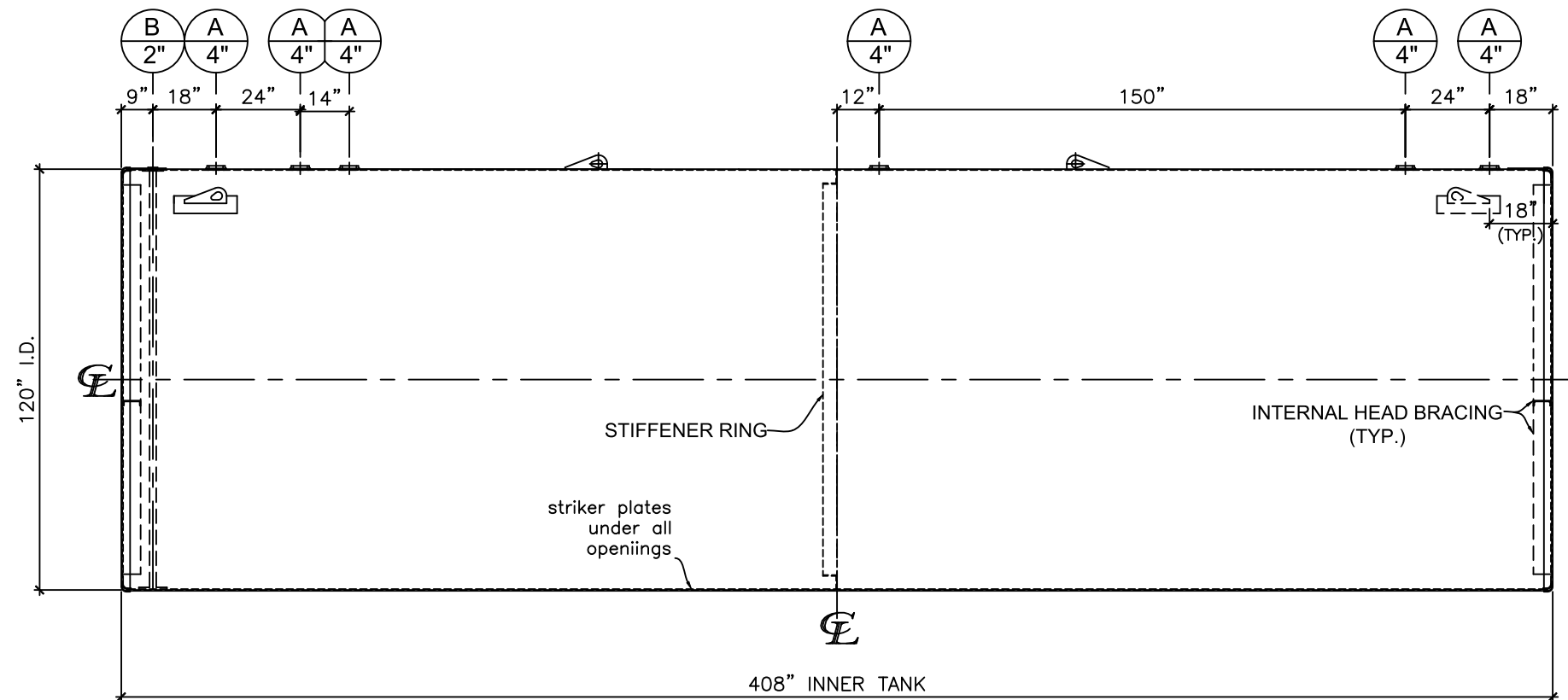
FRONT VIEW
