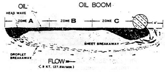
FIGURE 1-11 CONFIGURATION OF OIL AGAINST BOOM
