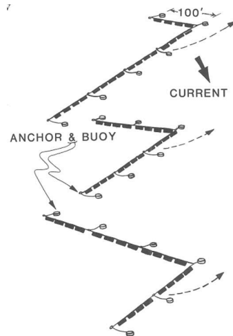
FIGURE 1-5 ANCHORING BOOMS AT 100-FT.
