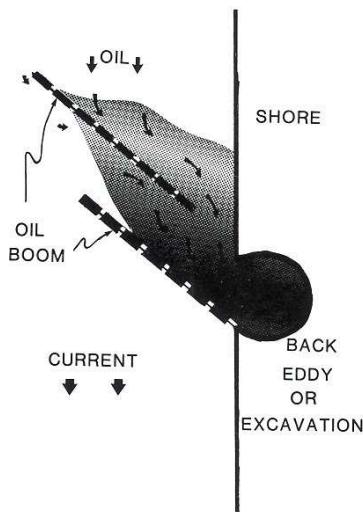
FIGURE 1-9 DOUBLE BOOMING USING BACK EDDIES
